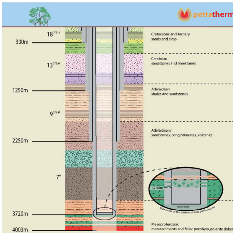
Figure 1 - Paralana 2 well, simplified geology and schematic of perforation zone
