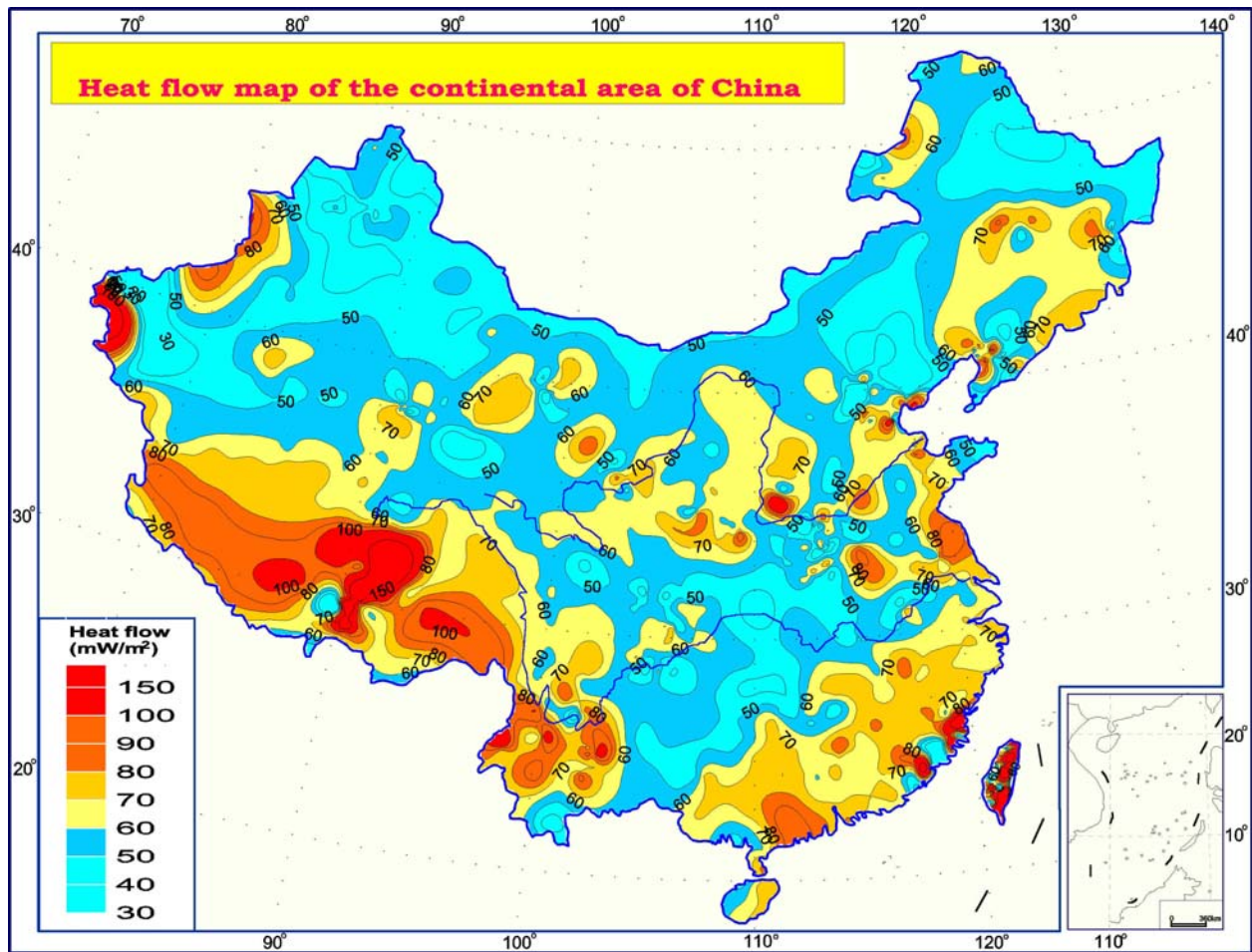
Figure 1 - Heat Flow Map of China (source: Professors Hu Shengbiao, He Lijuan and Wang Jiyang. 2000 – Chinese Academy of Sciences – Institute of Geology and Geophysics)
